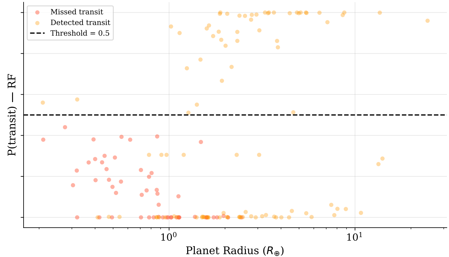
RF — Transit Score vs. Radius
