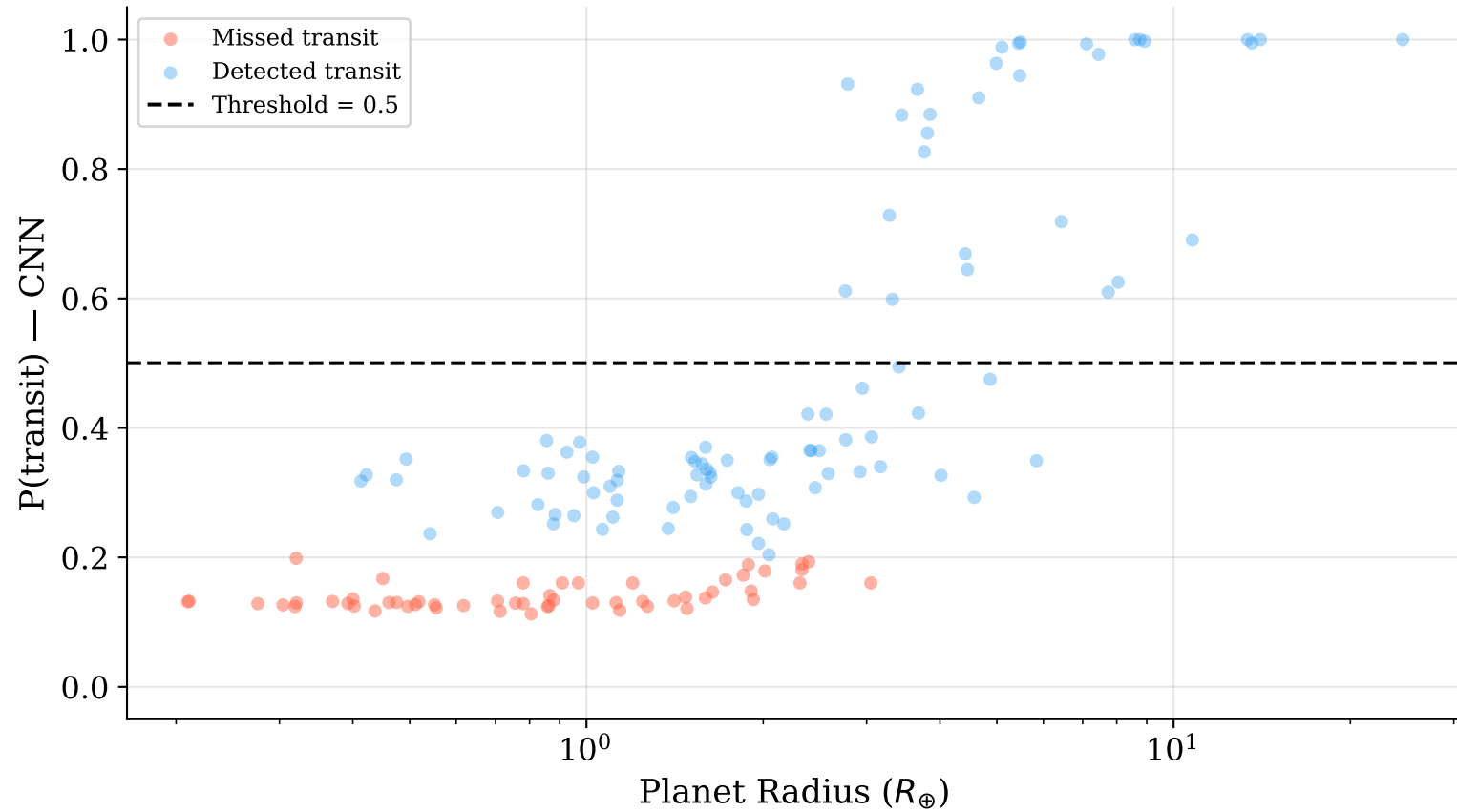
CNN — Transit Score vs. Radius
