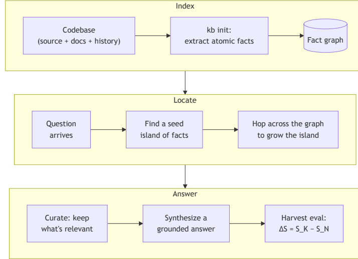
Figure 1: End-to-end KB system. Primary harvest grade: \Delta S (K vs. real agent); deep MOEL evaluation adds L_{\text{MOEL}} under toy-tool N/K/O conditions.
