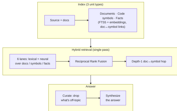
Figure 2: KB indexing (top) feeds the hybrid retriever: six lexical/neural lanes over documents, symbols, and facts are fused by Reciprocal Rank Fusion, a depth-1 doc↔symbol hop enriches the pool, and a curator prunes before one-shot synthesis (bottom).
