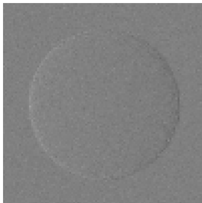
UMPA
