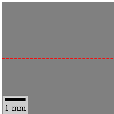
Ground Truth
