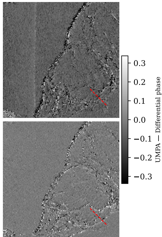
UMPA
