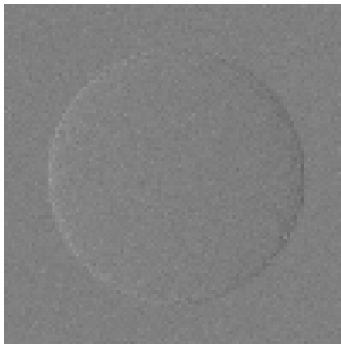
UMPA
