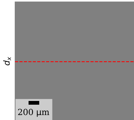
Ground Truth
