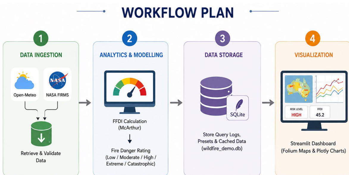
Figure 3: Workflow Plan
