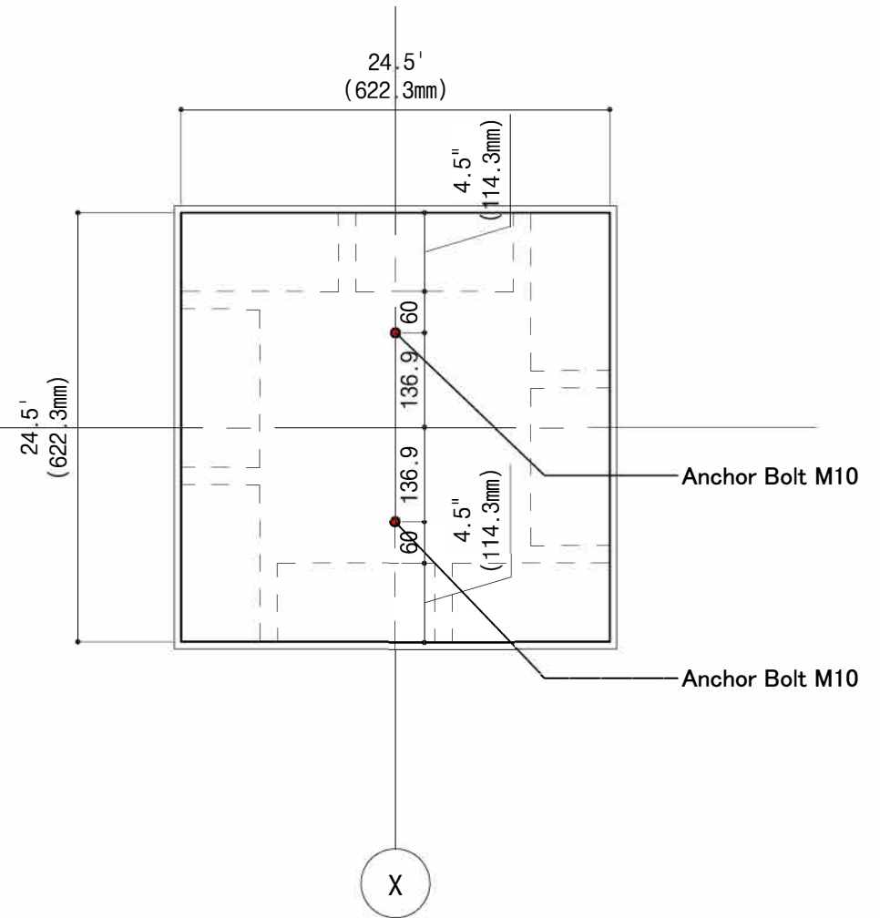
Anchor Bolt Detail Type A+B
