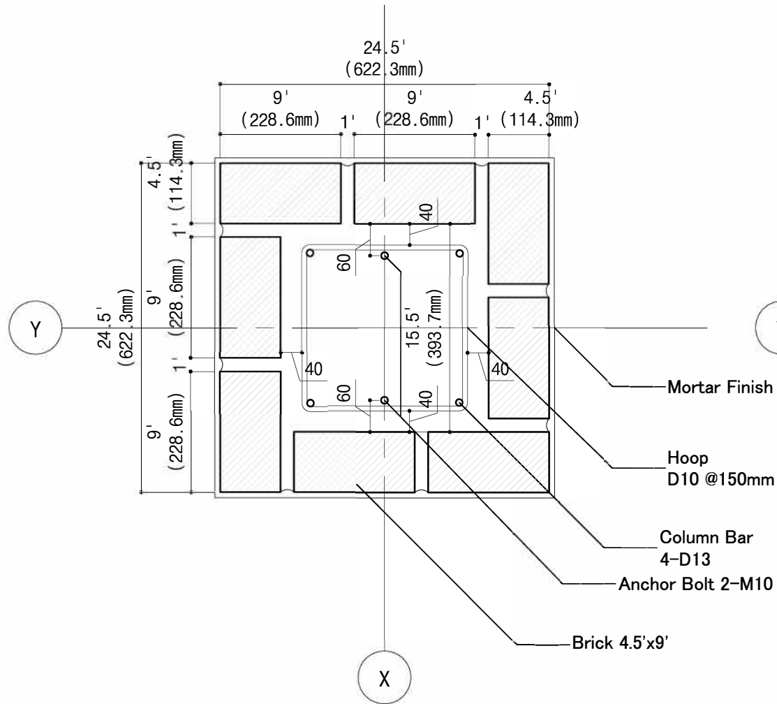
Reinforcement Detail Type A+B
