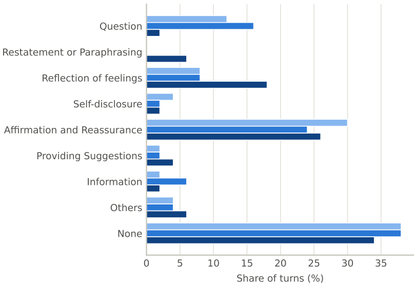
MultiAgentESC: predicted strategies (50 turns)
