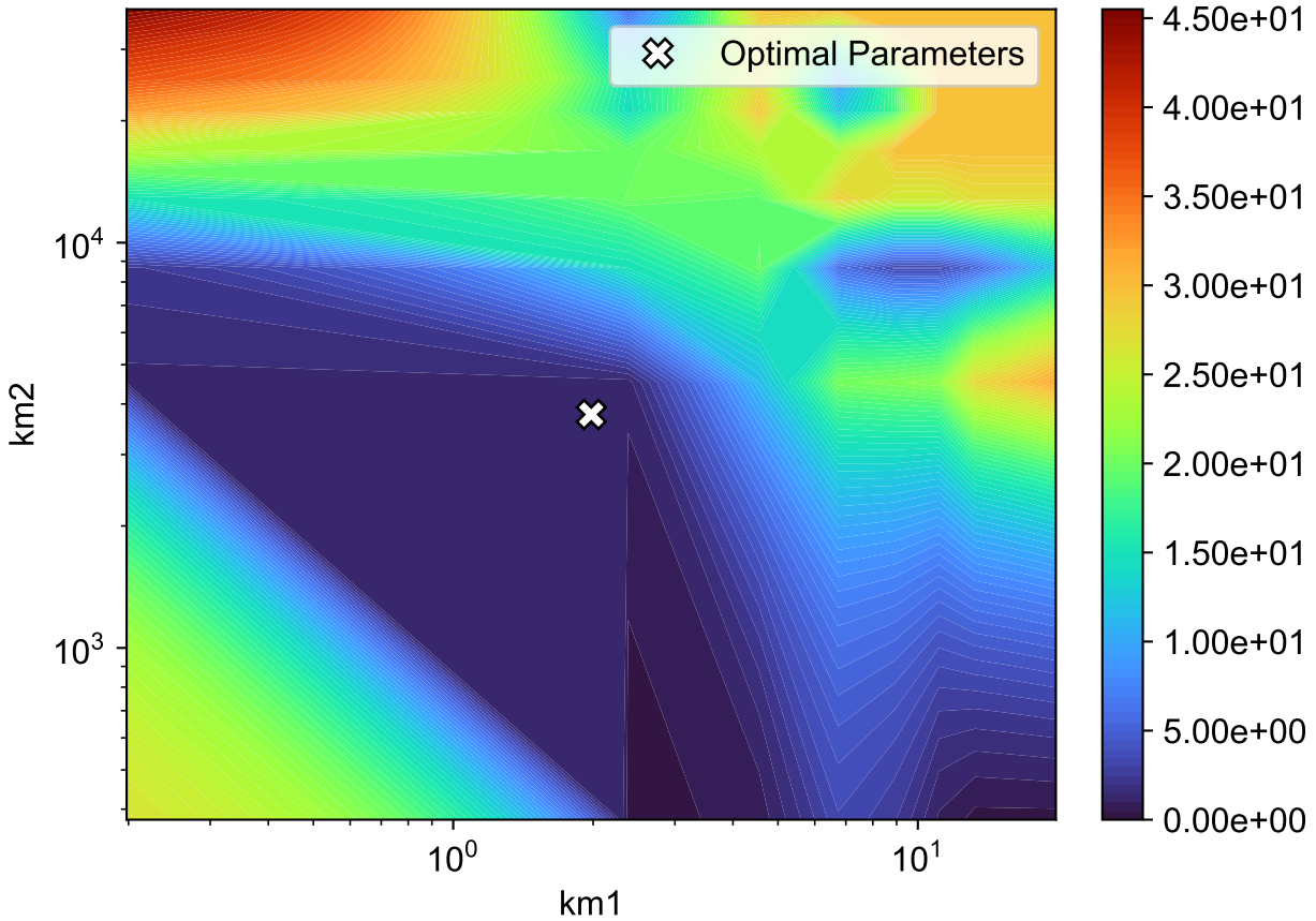
Parameter correlation surface for km1,km2
