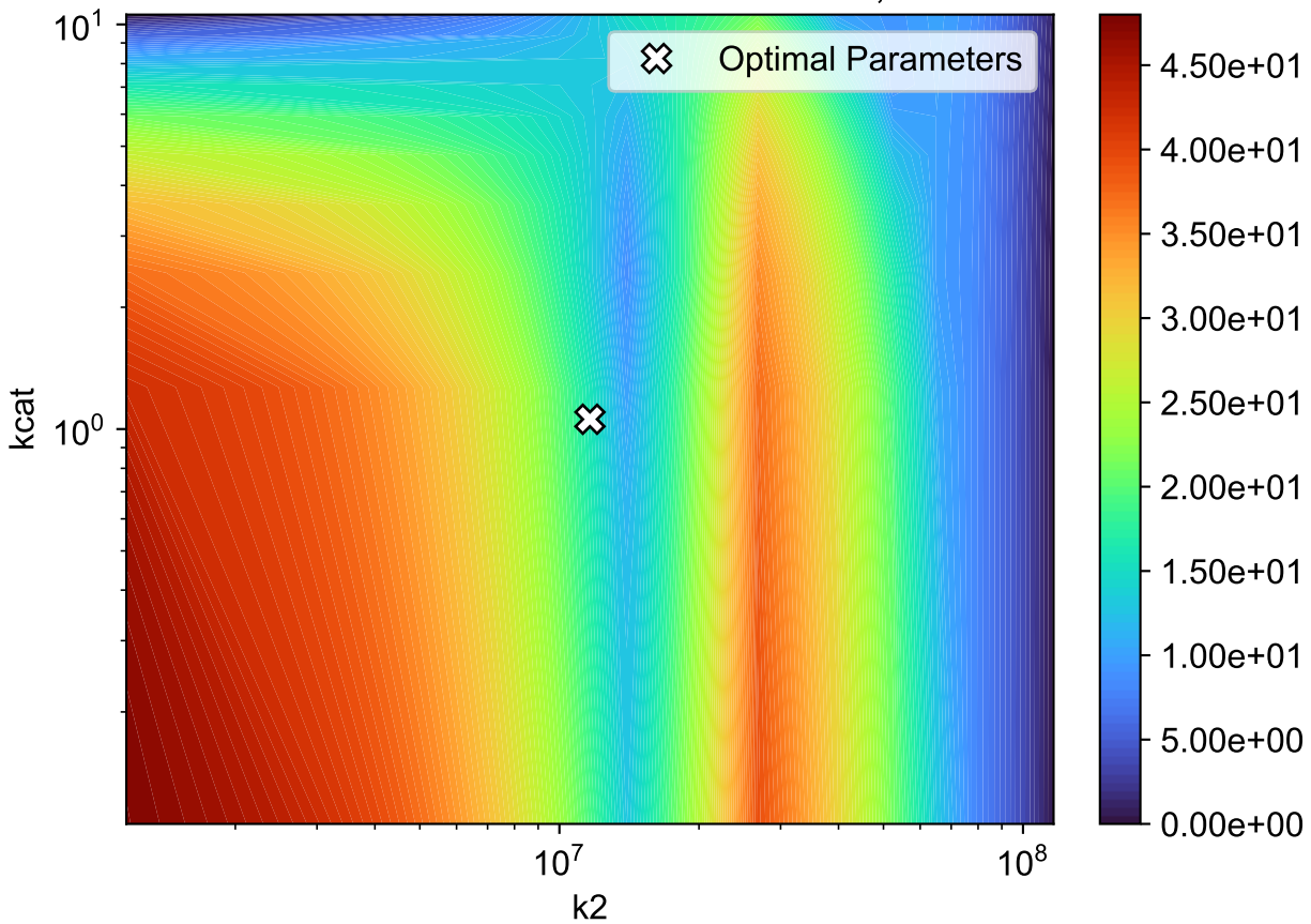
Parameter correlation surface for k2,kcat
