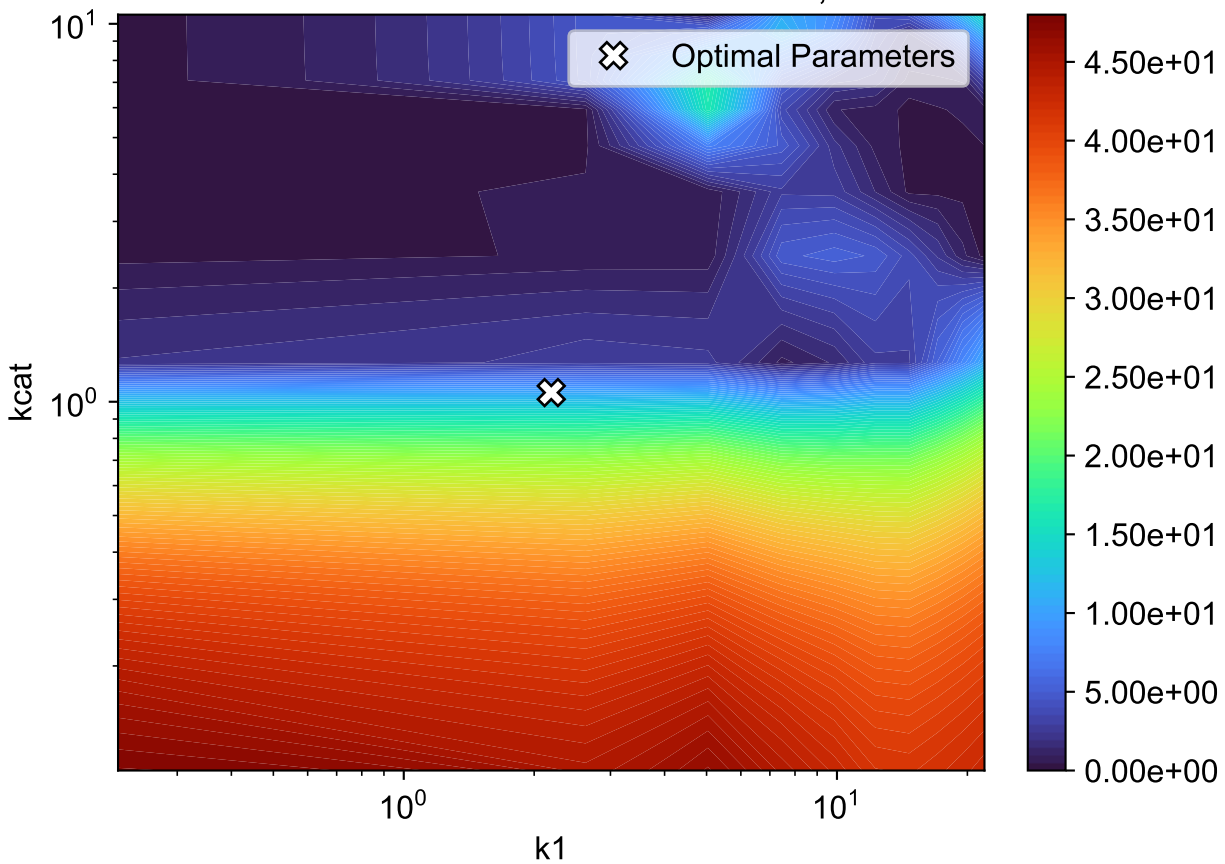
Parameter correlation surface for k_1, k_{cat}
