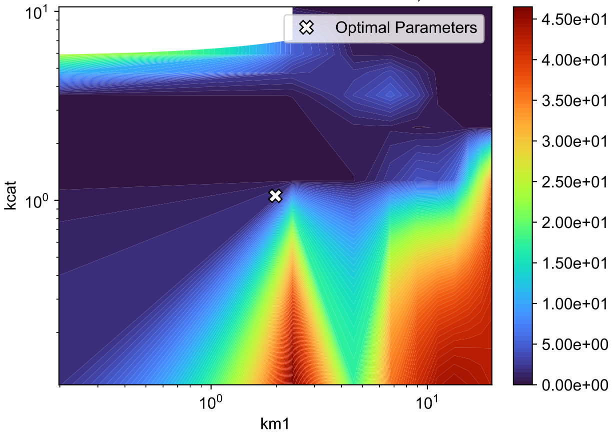
Parameter correlation surface for km1,kcat
