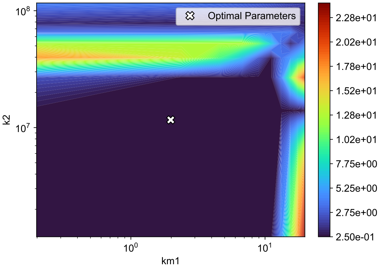
Parameter correlation surface for km1,k2
