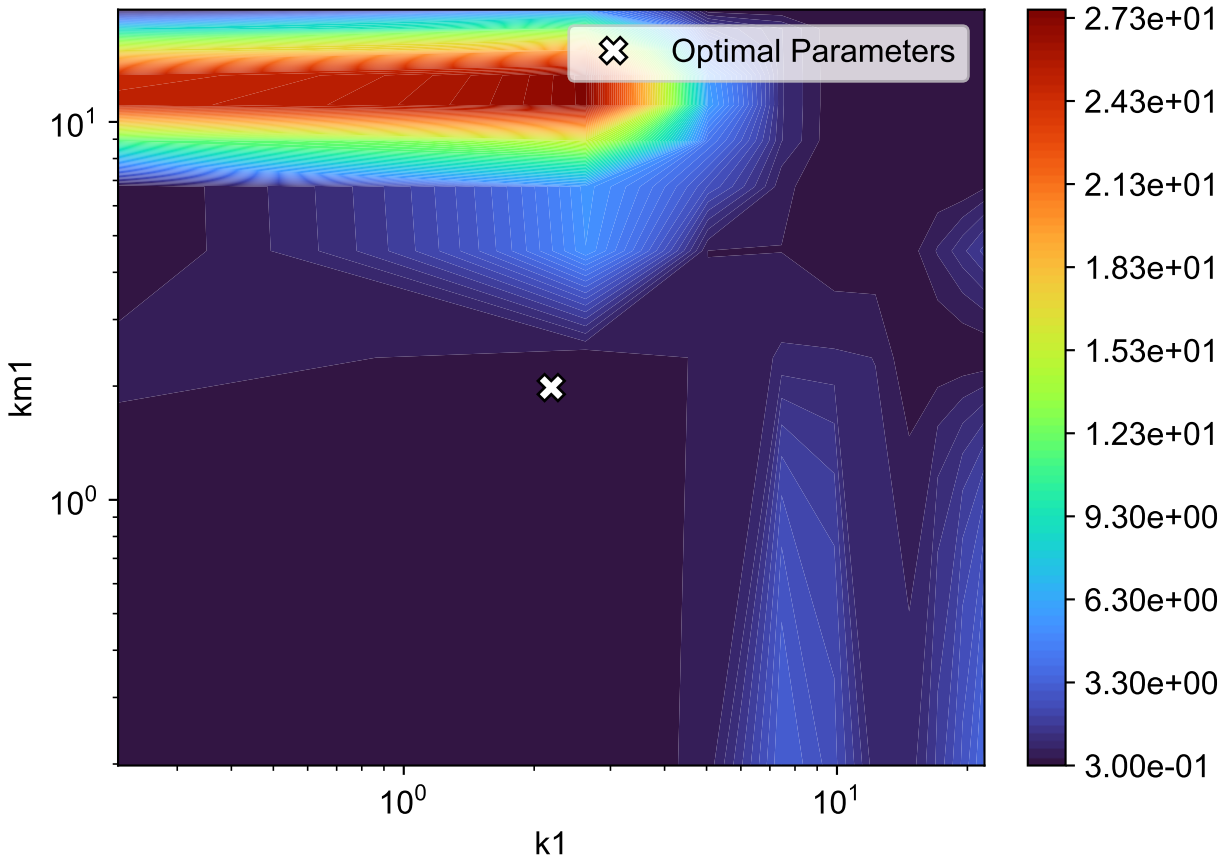
Parameter correlation surface for k_1, km_1
