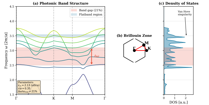
FIG. 1. Photonic band structure of the C_{6v} hexagonal lattice computed via plane-wave expansion. Shaded region indicates the complete TM band gap ( \Delta\omega/\omega_{\text{mid}} = 21\% ).
