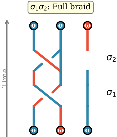
(a) Anyon Braiding Worldlines
