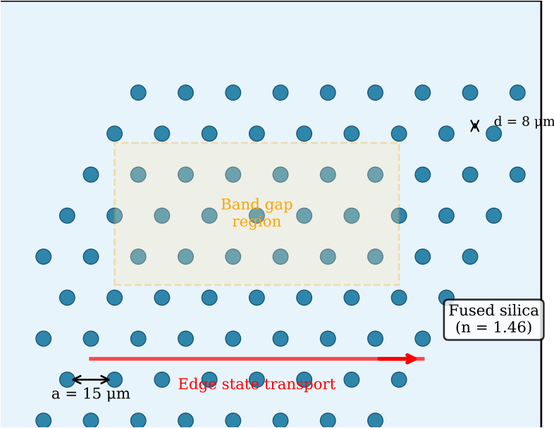
(b) Hexagonal Photonic Crystal (Top View)
