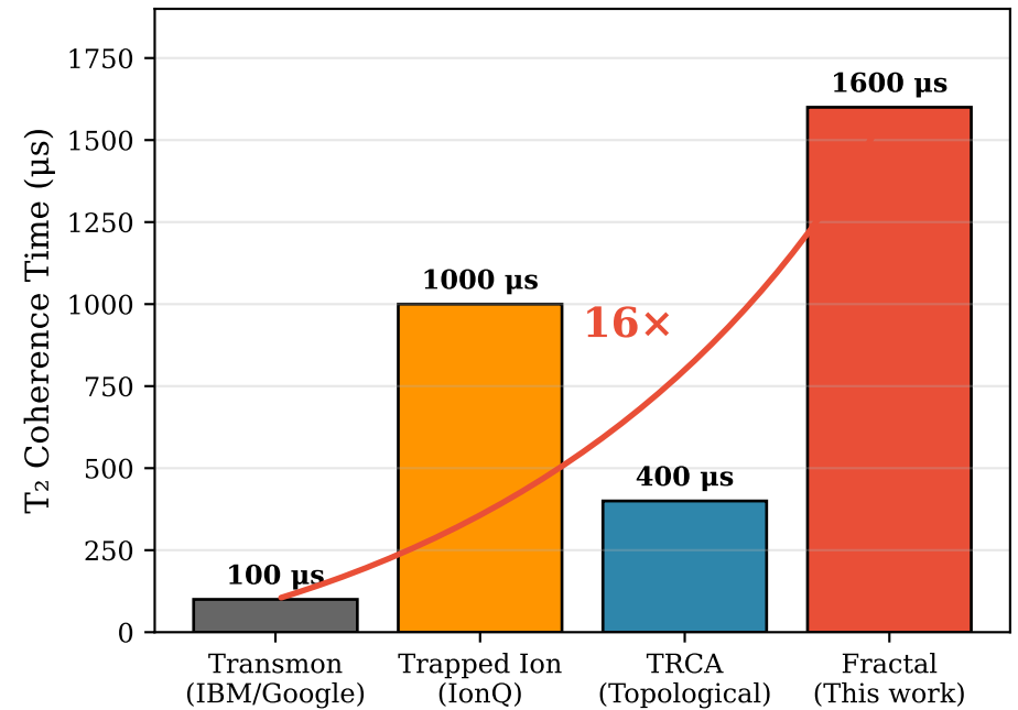
(b) Coherence Time Comparison
