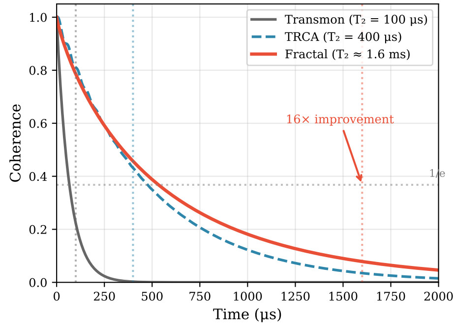
(a) Coherence Decay: Transmon vs TRCA vs Fractal
