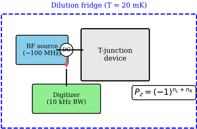
(c) RF Reflectometry Setup
