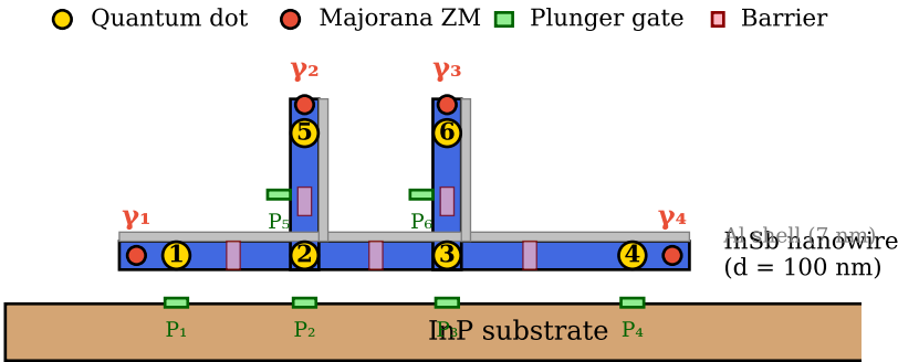
(a) T-Shape 6-Dot Majorana Device
