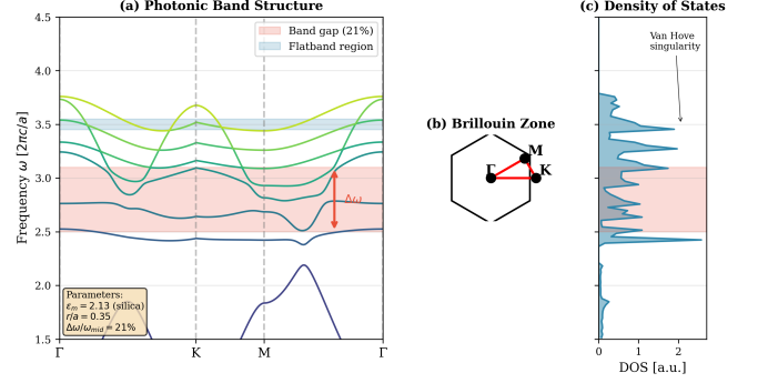
FIG. 2. Photonic band structure of the C_{6v} hexagonal lattice along \Gamma - K - M - \Gamma . The 21.4% complete band gap (shaded) spans \omega_1 = 2.50 to \omega_2 = 3.10 (in units of 2\pi c/a ). Flatband regions near \omega = 3.50 support Anderson localization.
