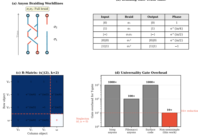
FIG. 3. Neglecton braiding diagram showing worldlines of neglecton \omega and semisimple anyon a . The non-trivial R -matrix phase R_{\omega,a} = e^{i\pi/4} enables universal gate generation.
