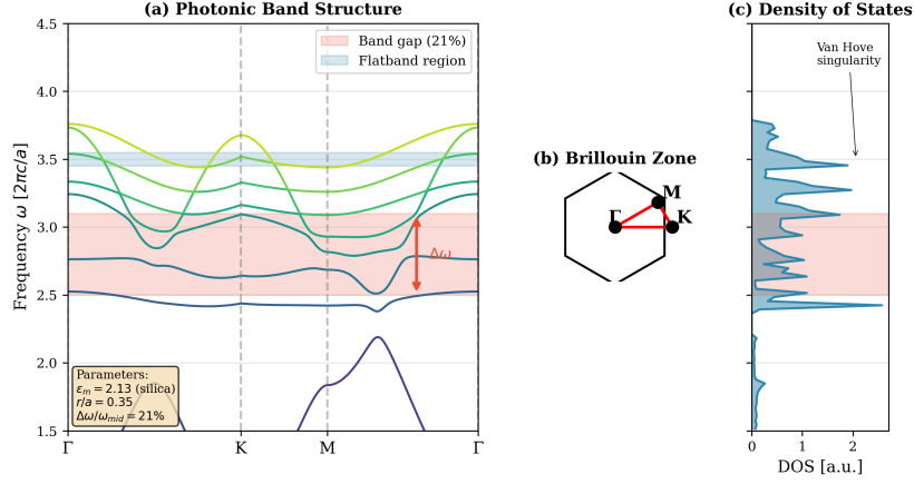
Figure 2: Photonic band structure showing complete gap and flatband modes.
