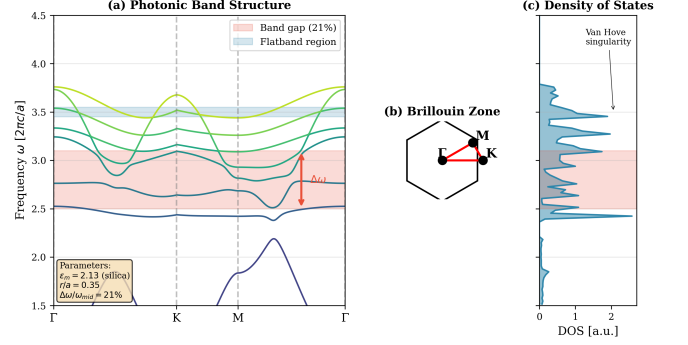
FIG. 2. Photonic band structure of the C_{6v} hexagonal lattice along \Gamma-K-M-\Gamma . The 21.4% complete band gap (shaded) spans \omega_1 = 2.50 to \omega_2 = 3.10 (in units of 2\pi c/a ). Flatband regions near \omega = 3.50 support Anderson localization.
