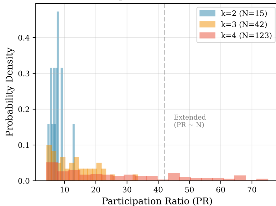
(b) Participation Ratio Distribution
