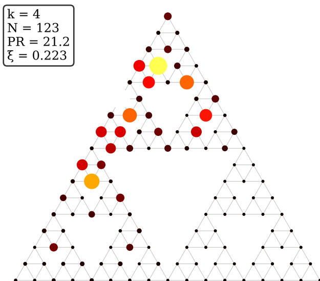
(a) Localized Wavefunction (k=4)
