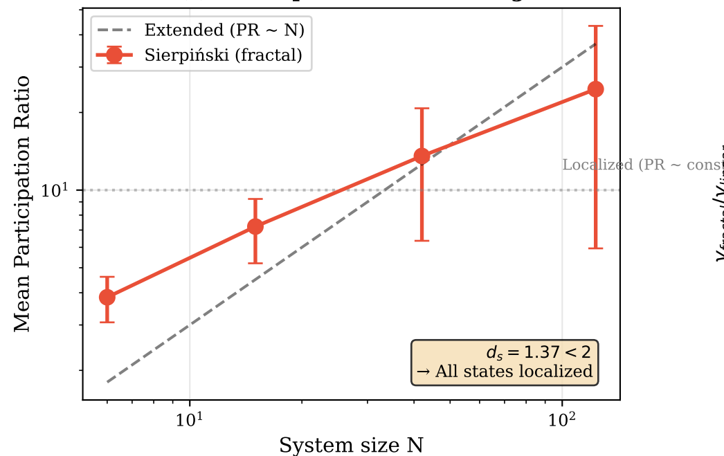
(c) Participation Ratio Scaling
