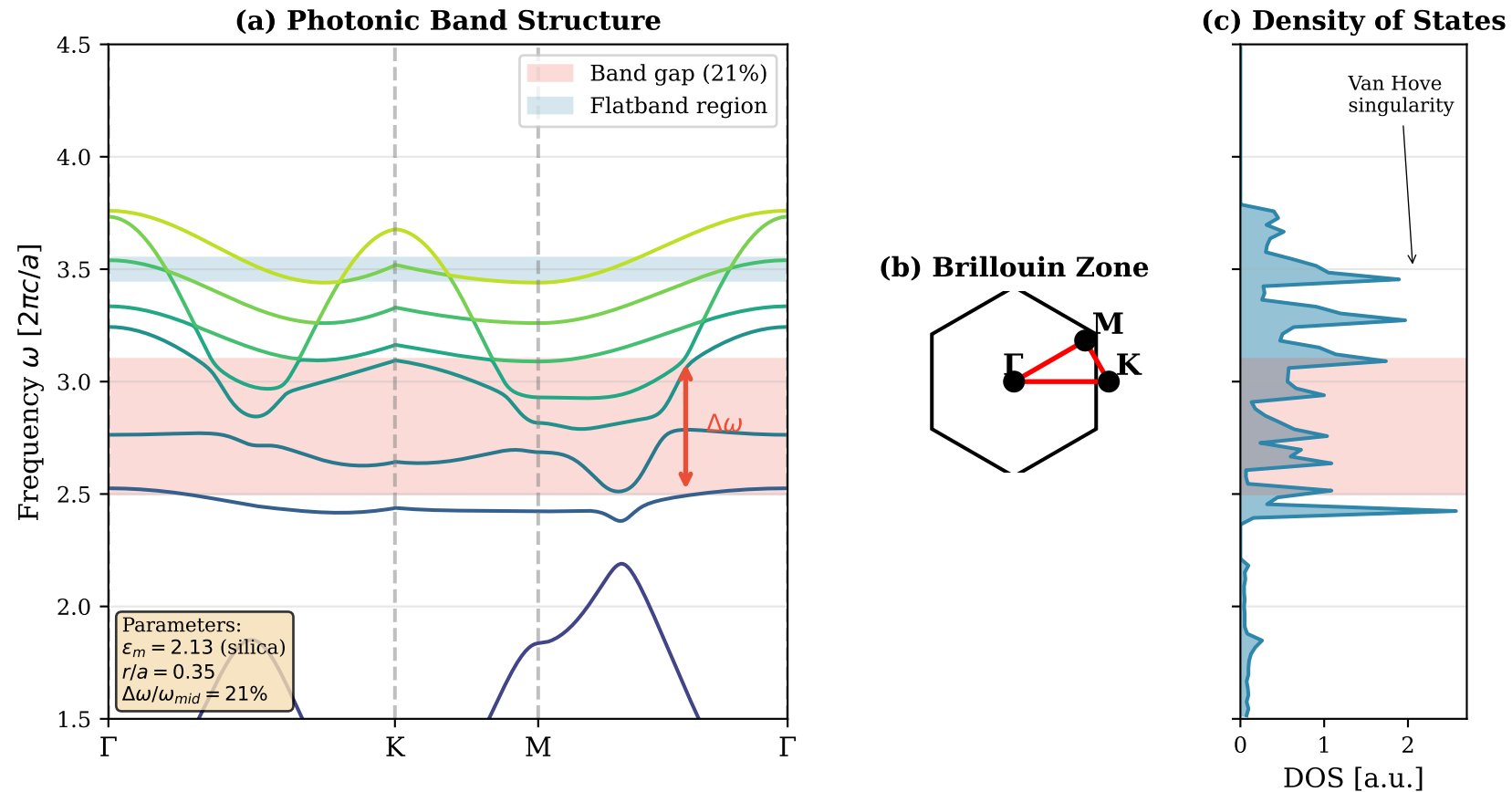
Figure 5: C_{6v} Hexagonal Photonic Crystal Band Structure
