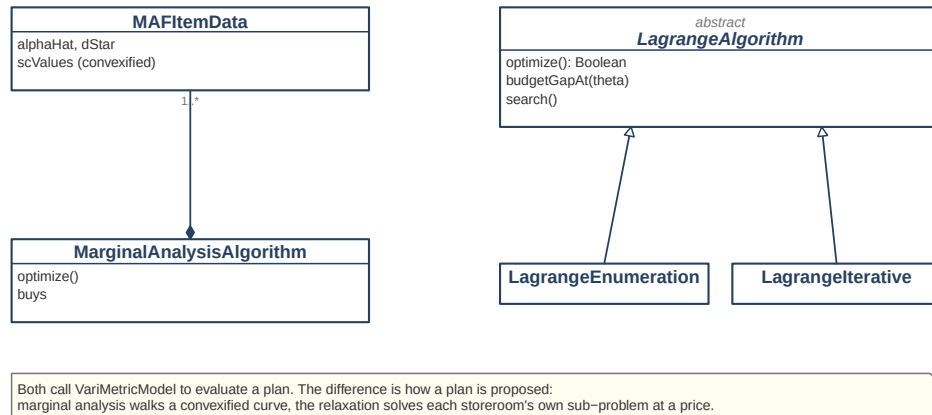
Figure 9.11.: The two families of search. Marginal analysis builds a curve for each item and then merges the curves; the relaxation prices money and hunts for the price that spends the budget. LagrangeAlgorithm holds everything except how the multiplier is chosen, which is the one method its two subclasses supply. Notice that both families end up calling the same evaluation, so neither is a different model.
