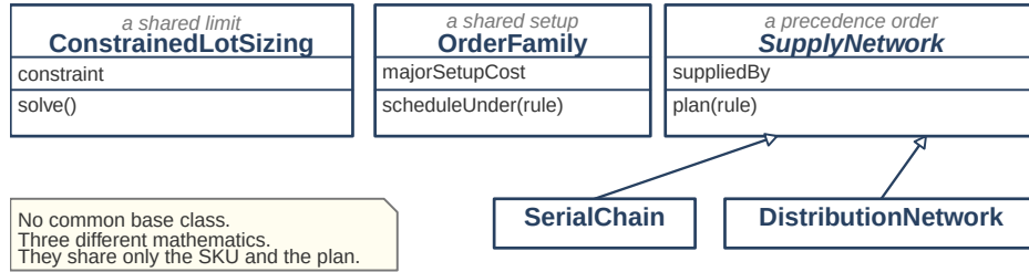
Figure 4.19.: The three couplings of this chapter as three unrelated classes. A shared limit, a shared setup and a precedence order are different mathematics, so they have no common supertype. The two network topologies do share one, since they differ only in the shape of a single map.
