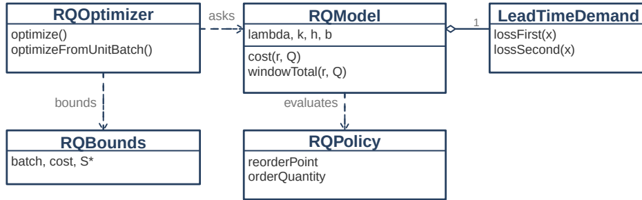
Figure 8.12.: The concepts of this chapter before any thought about implementation. An item holds a lead time demand distribution and evaluates any policy against it. An optimizer reads the item, asks it for the bounds of Section 8.9, and returns a policy. Notice that the optimizer holds no state of the item's: everything it needs it asks for, which is what allows two different searches to be run against one item and compared.
