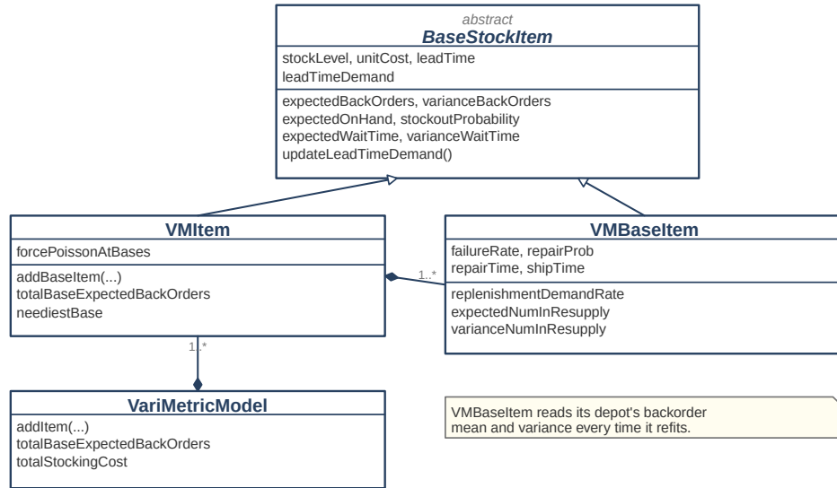
Figure 9.10.: The evaluation classes. Everything a location can be asked lives in BaseStockItem , because Equation 9.5 says the net inventory is the stock level minus the units in resupply and nothing else enters. A depot and a storeroom are both locations and differ only in how they obtain their lead time demand: the depot by Palm's theorem directly, the storeroom by fitting two moments that include the depot's backorder variance. The composition runs the other way from the dependency, which is the coupling drawn twice.
