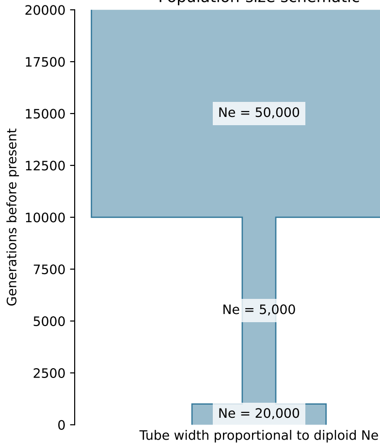
Population-size schematic
