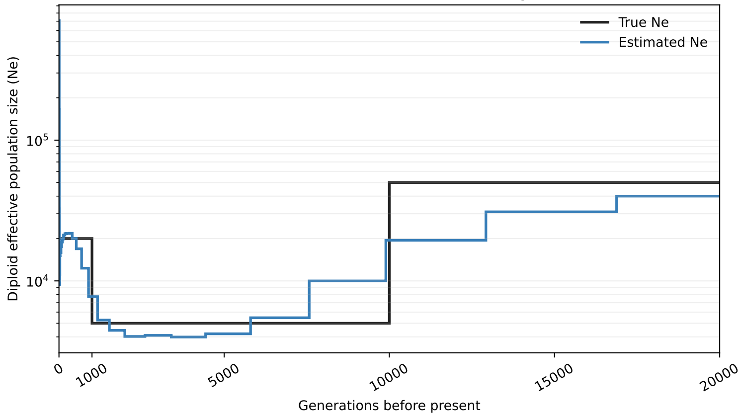
True and estimated Ne: most recent 20,000 generations
