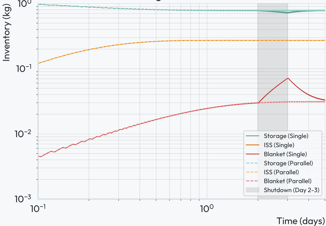
Tritium Inventories – Single vs Parallel BCRs with Shutdown
