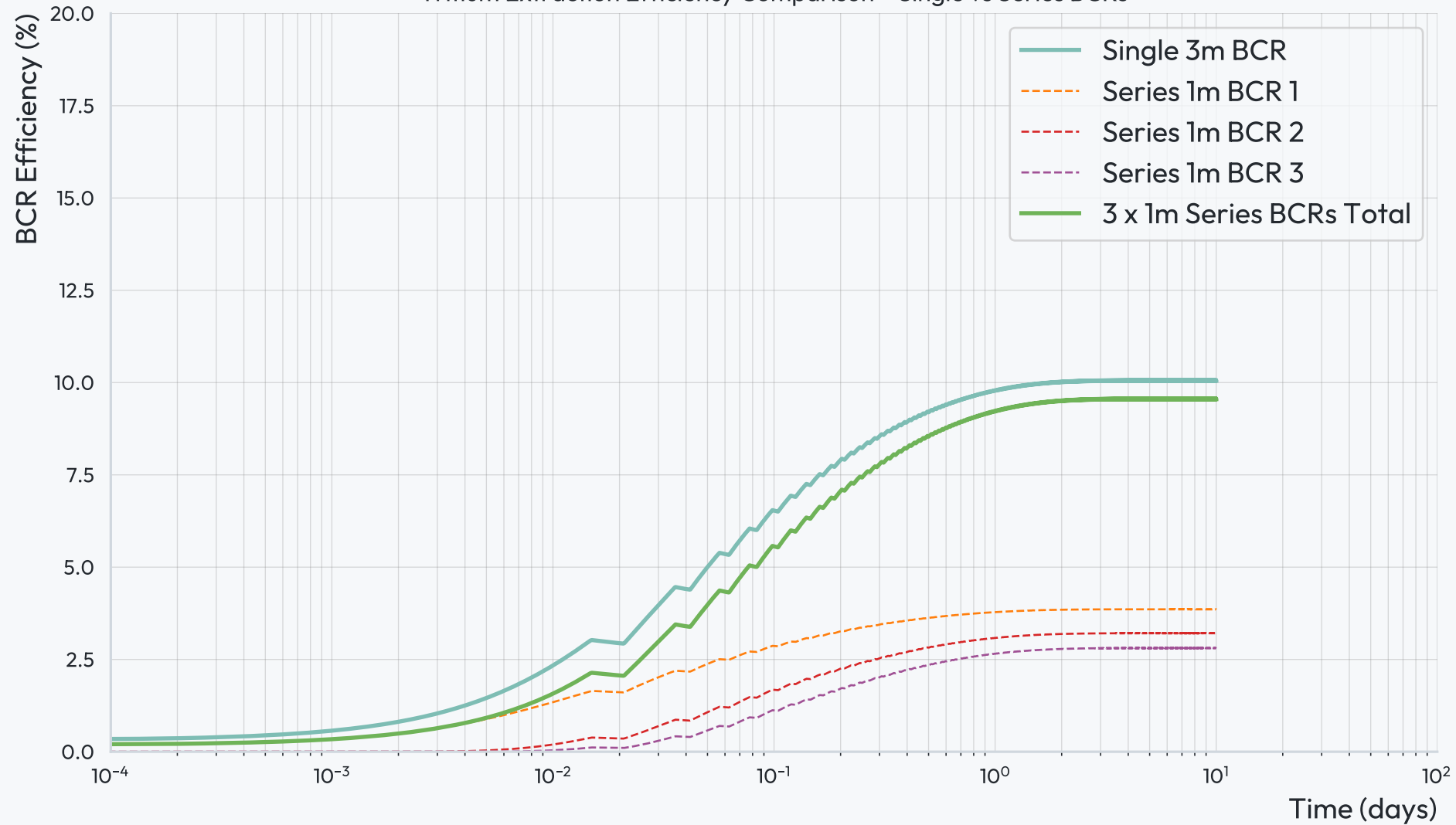
Tritium Extraction Efficiency Comparison – Single vs Series BCRs
