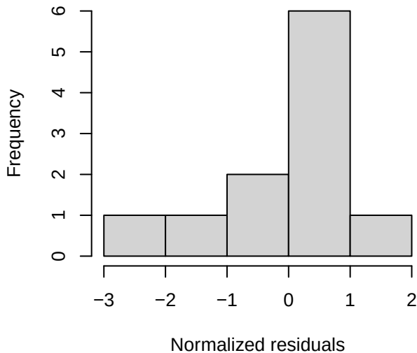
pgls_ctmax normalized residuals
