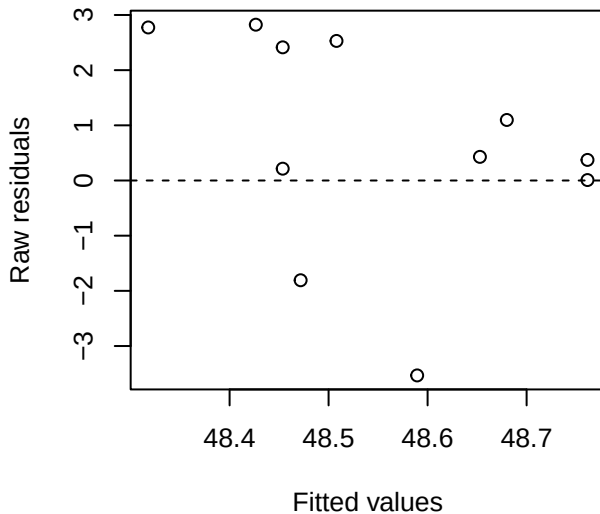
pgls_ctmax raw residuals vs fitted
