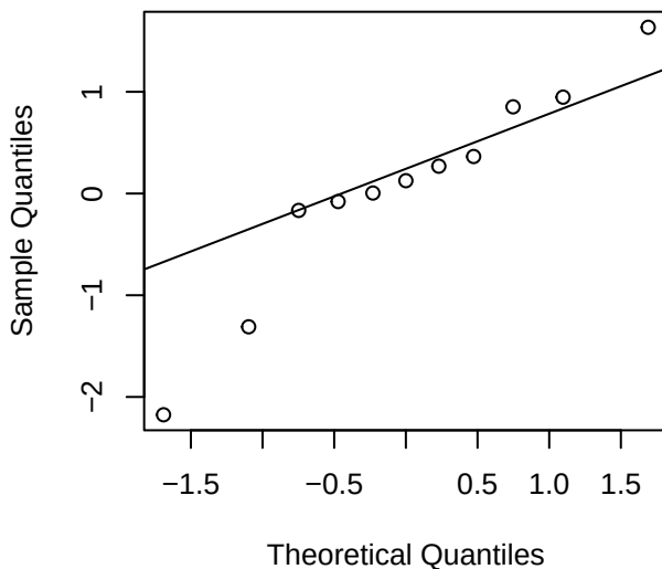
pgls_ctmax normal Q-Q
