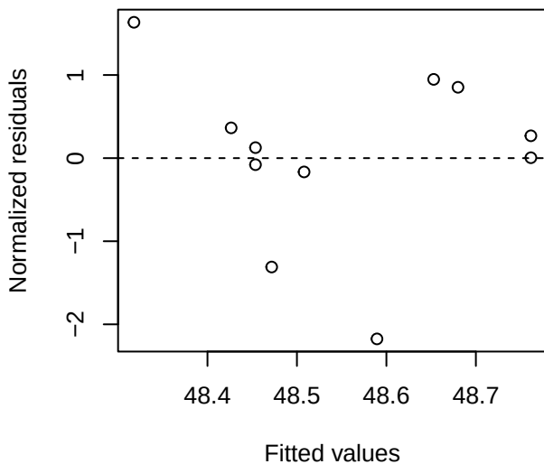
pgls_ctmax residuals vs fitted
