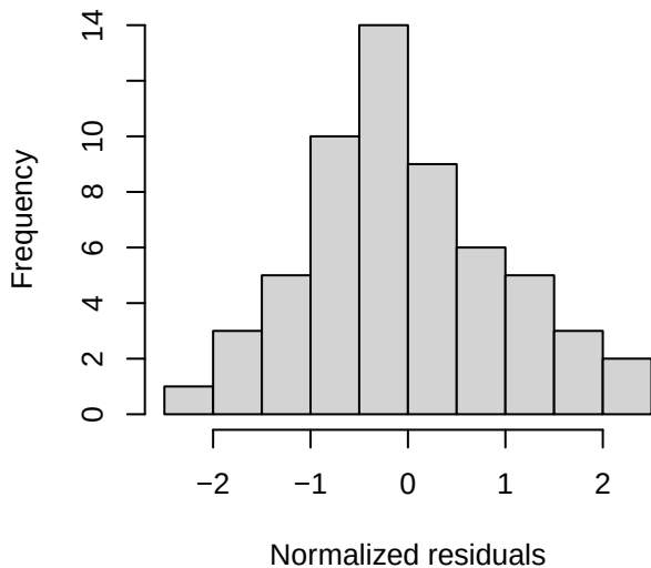
pgls_mass normalized residuals
