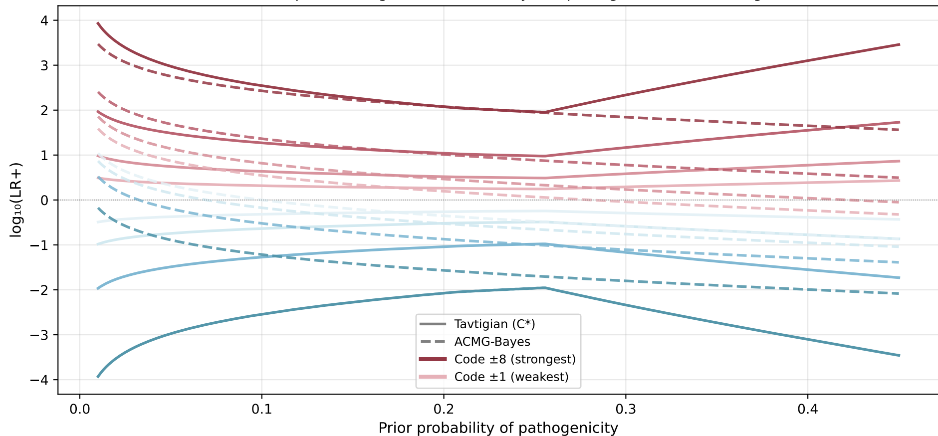
LR+ thresholds vs prior [Tavtigian (C*), ACMG-Bayes] (pathogenic above 0, benign below 0)
