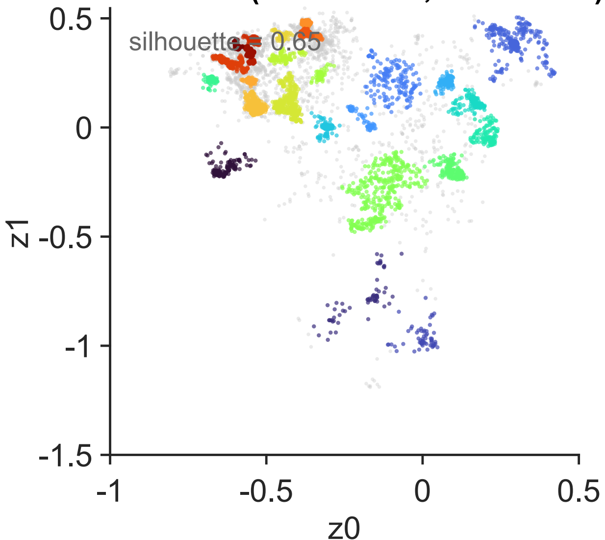
HDBSCAN (27 clusters, 14% noise)
