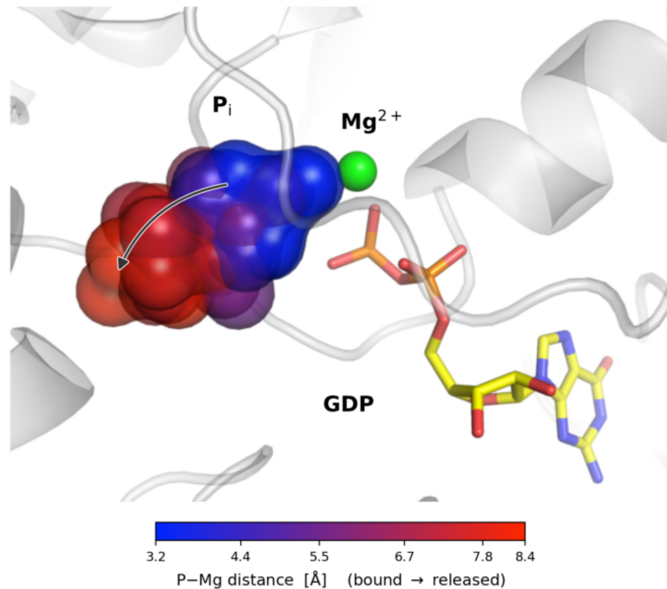
(a) Phosphate-release pathway
