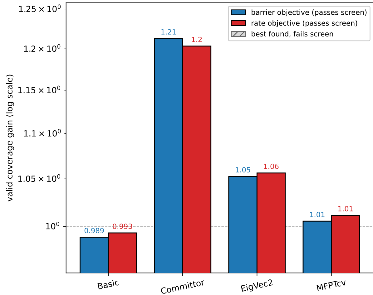
(b) Pentapeptide MSM ( n = 250 )
