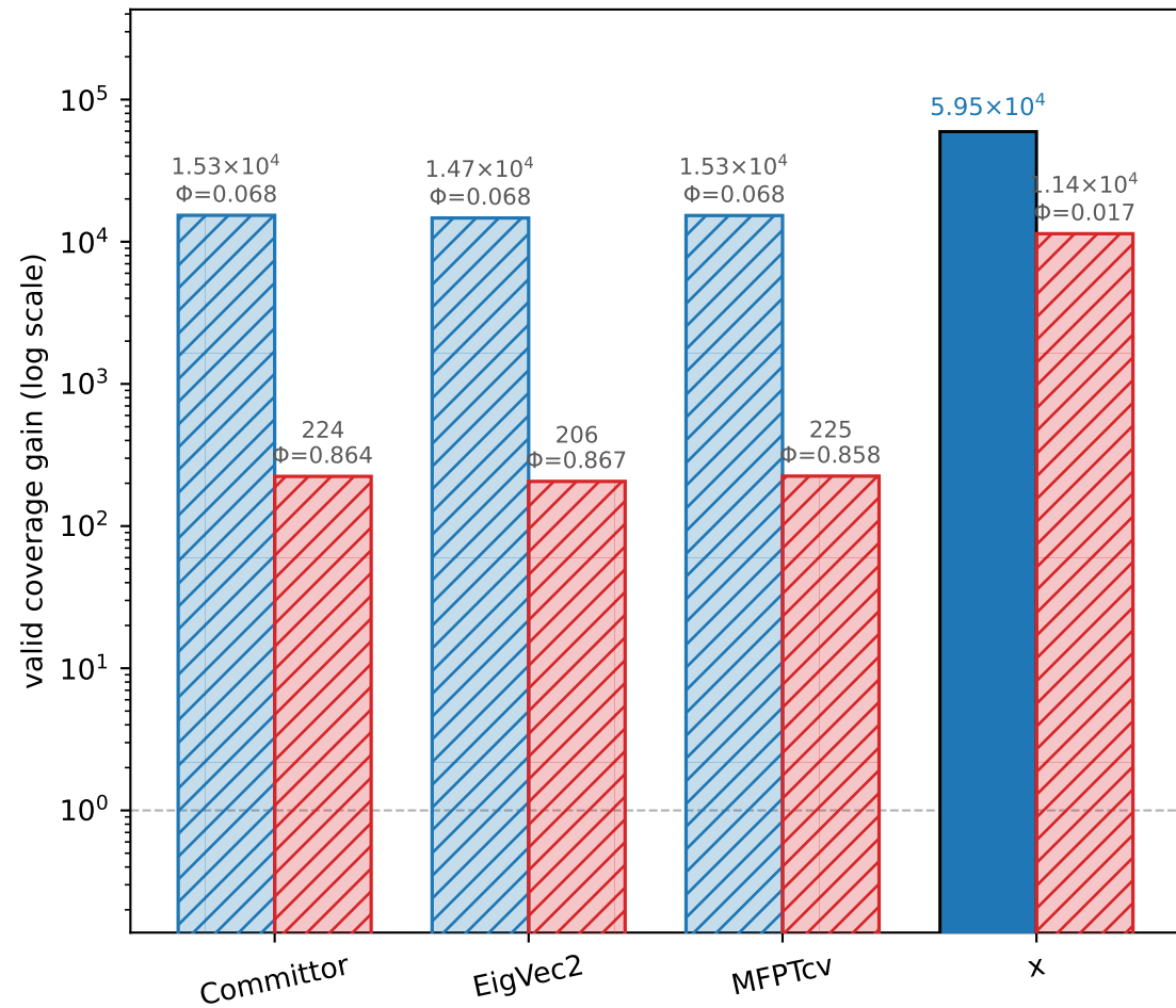
(a) 2D grid ( n = 800 , deep barrier)
