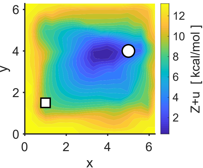
Spectral-opt U_{\max}=6 k_B T
