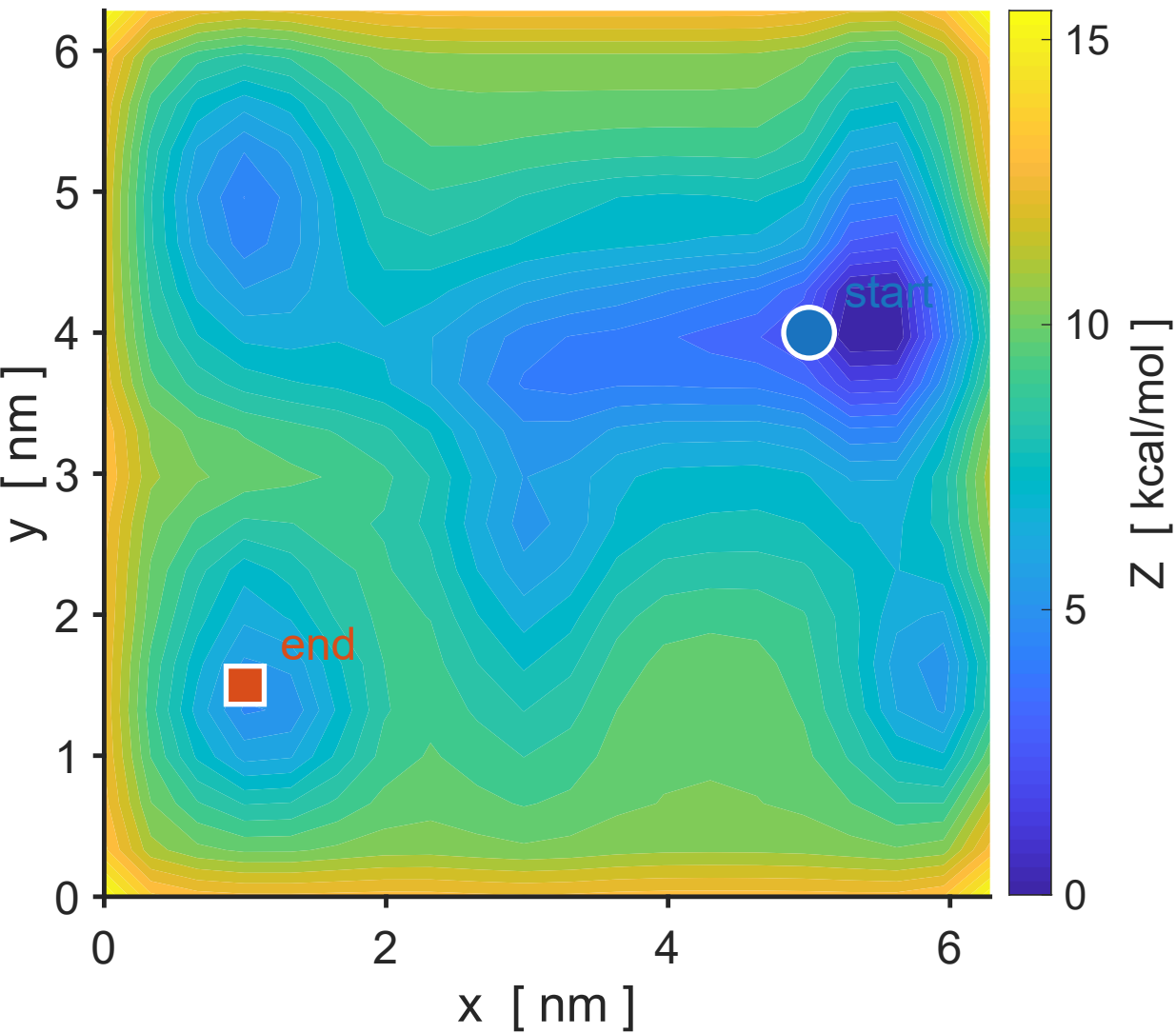
9-well landscape
