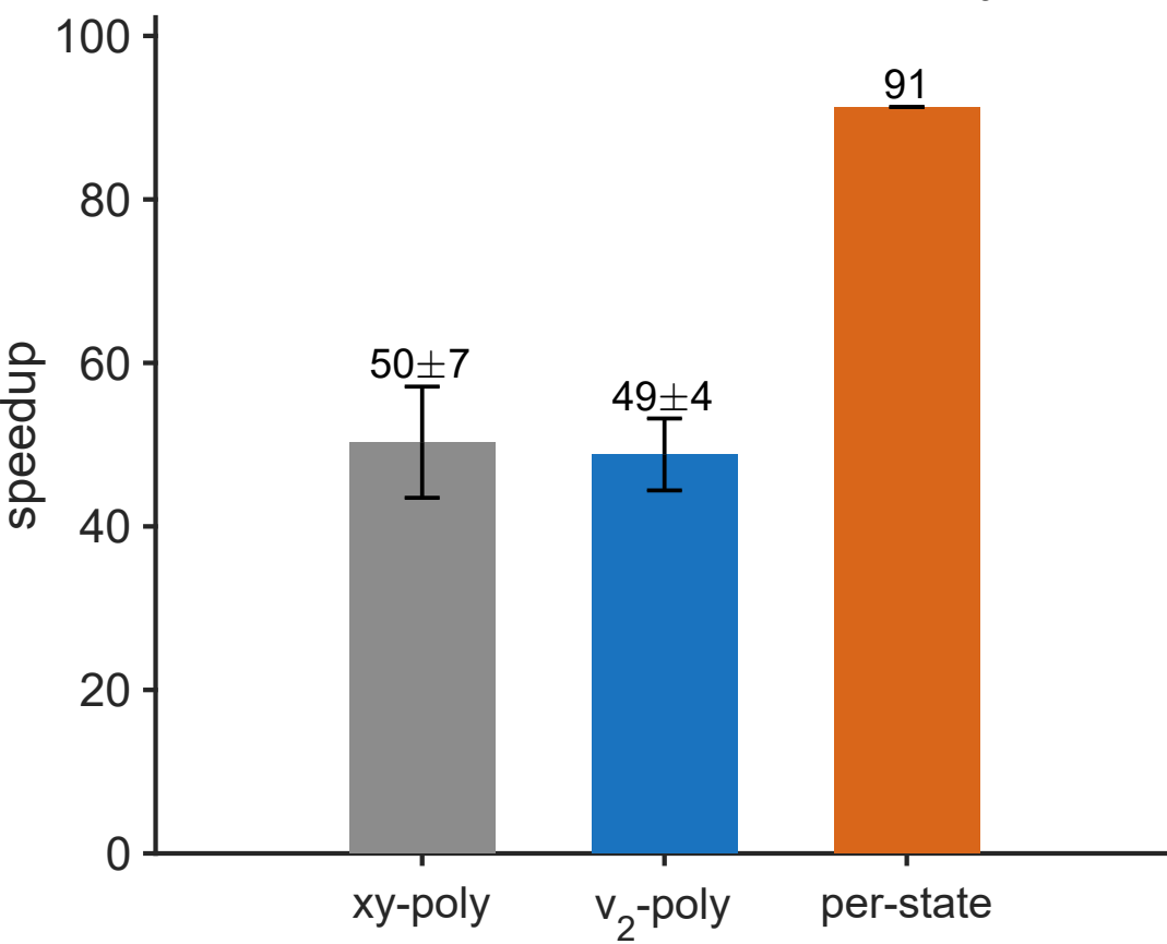
(a) spectral-gap speedup \gamma/\gamma_0
