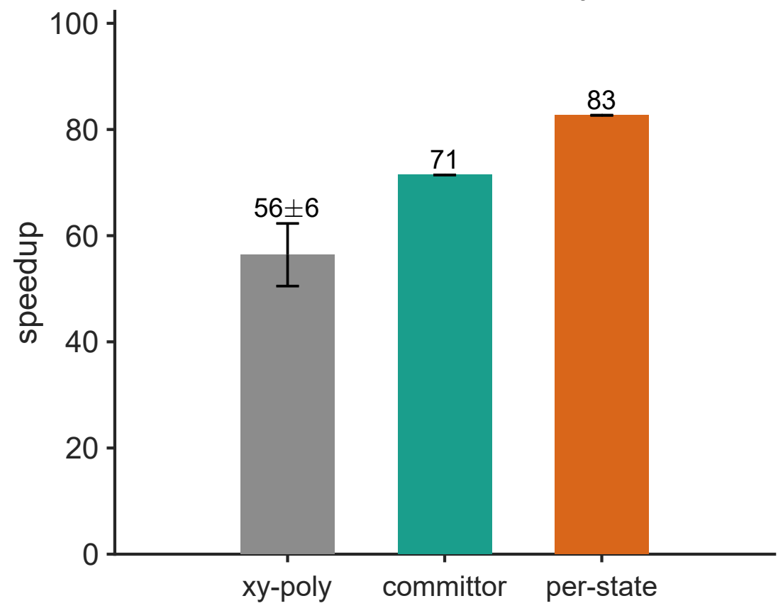
(b) MFPT speedup \tau_0/\tau
