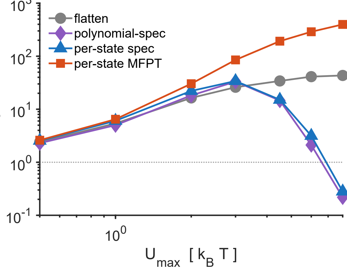
(b) MFPT speedup
