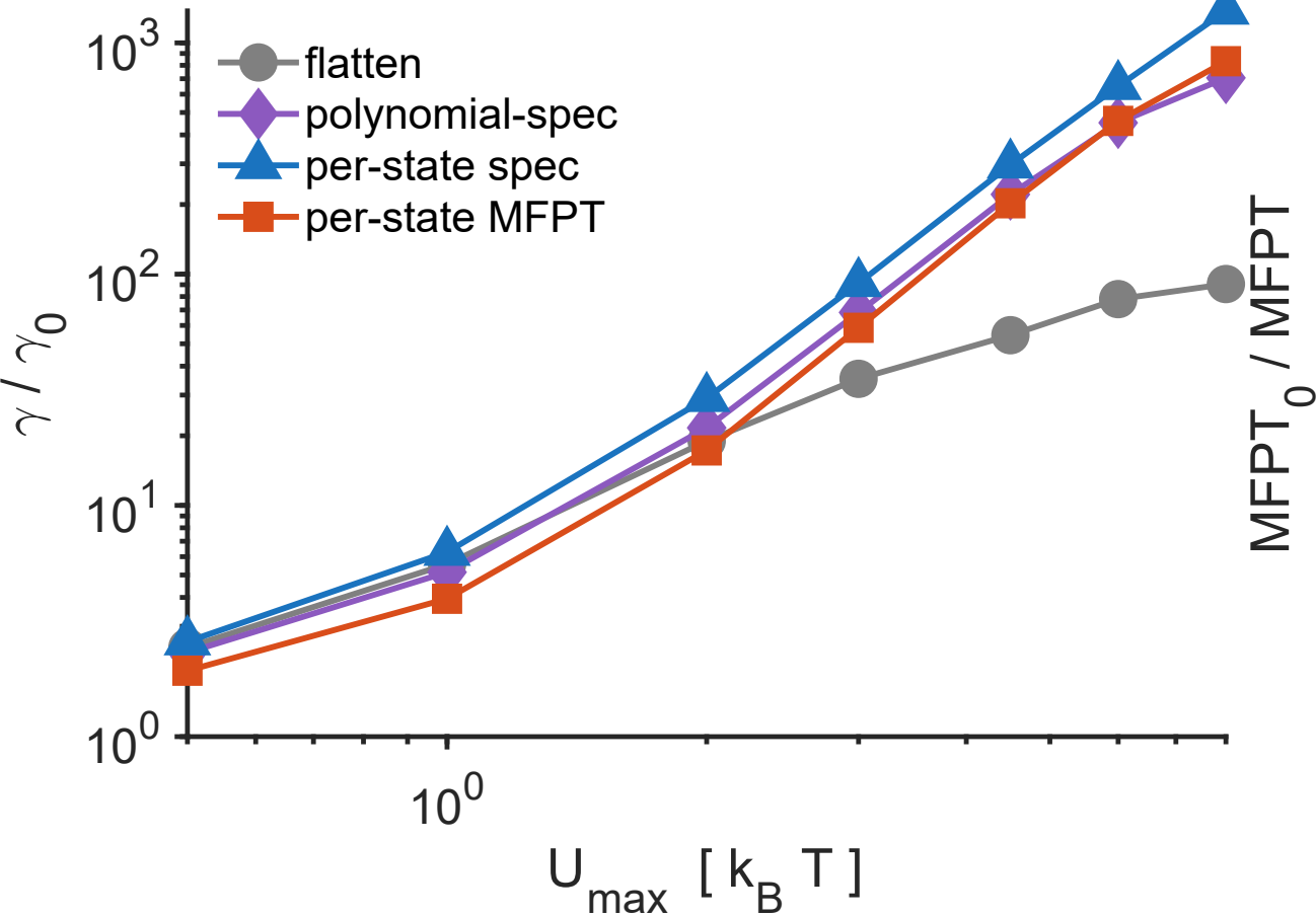
(a) Spectral-gap speedup
