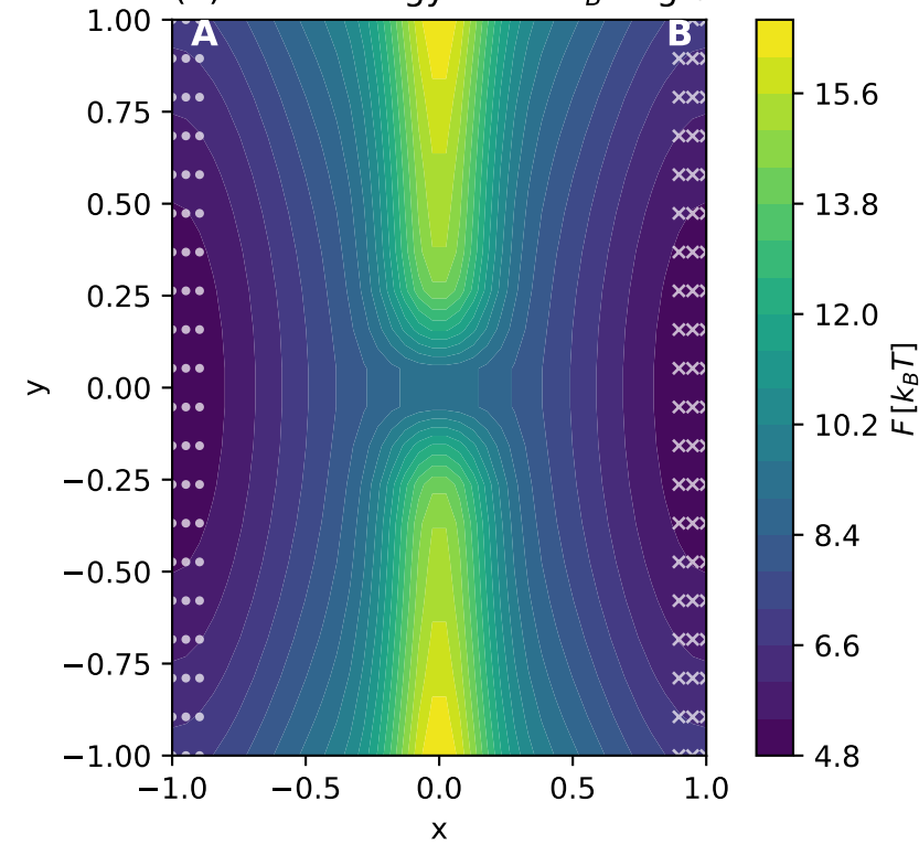
(a) Free energy F = -k_B T \log \pi
