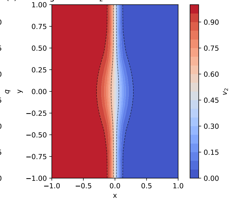
(c) Slow eigenvector v_2 with W = 4 umbrella centers
