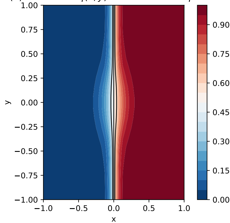
(b) Committor q(x, y) with band 0.4 < q < 0.6
