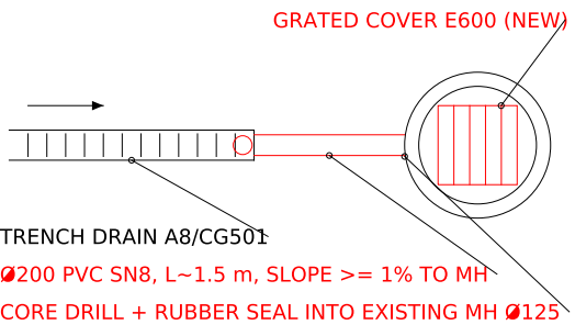
DETAIL 1 - TYPICAL CONNECTION (PLAN) ENLARGED APPROX. 1:80
