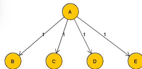
Graph 4 Visualization
