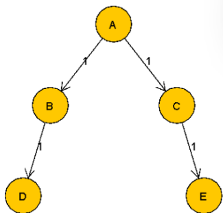
Graph 2 Visualization
