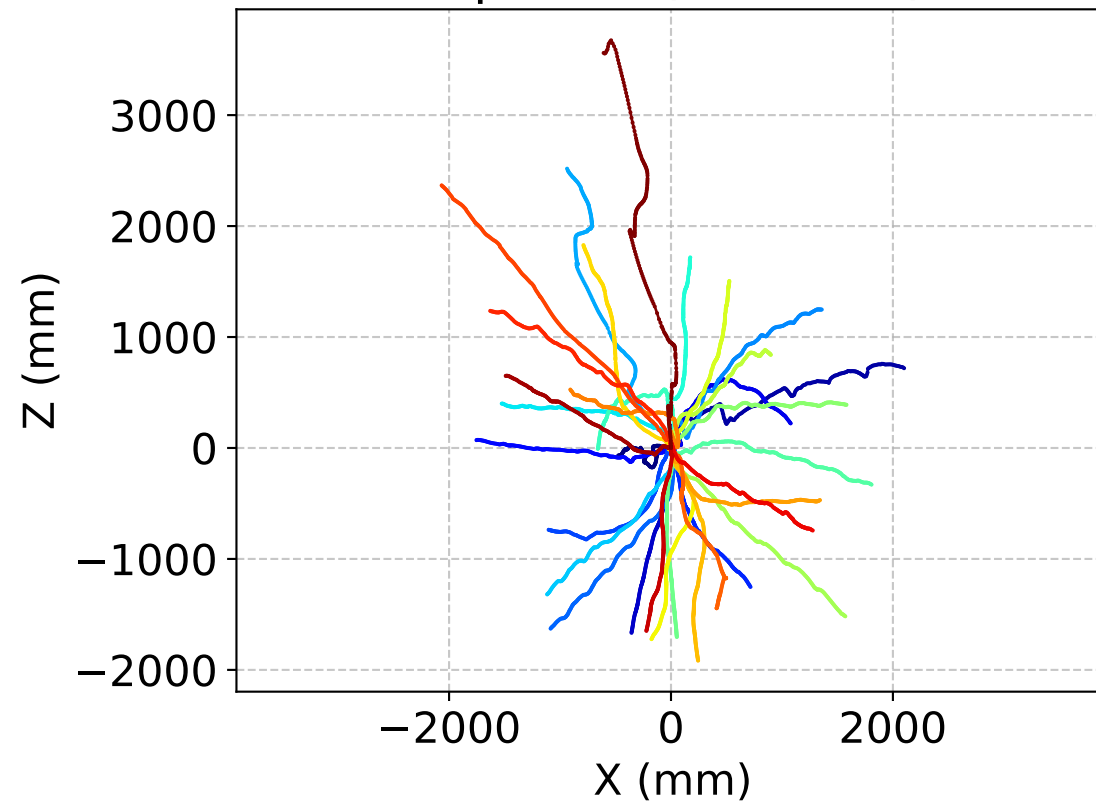
Top View (XZ Plane)
