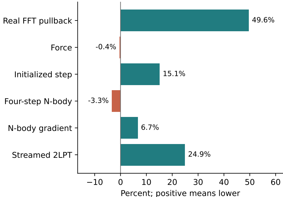
Compiler temporary-buffer reduction
