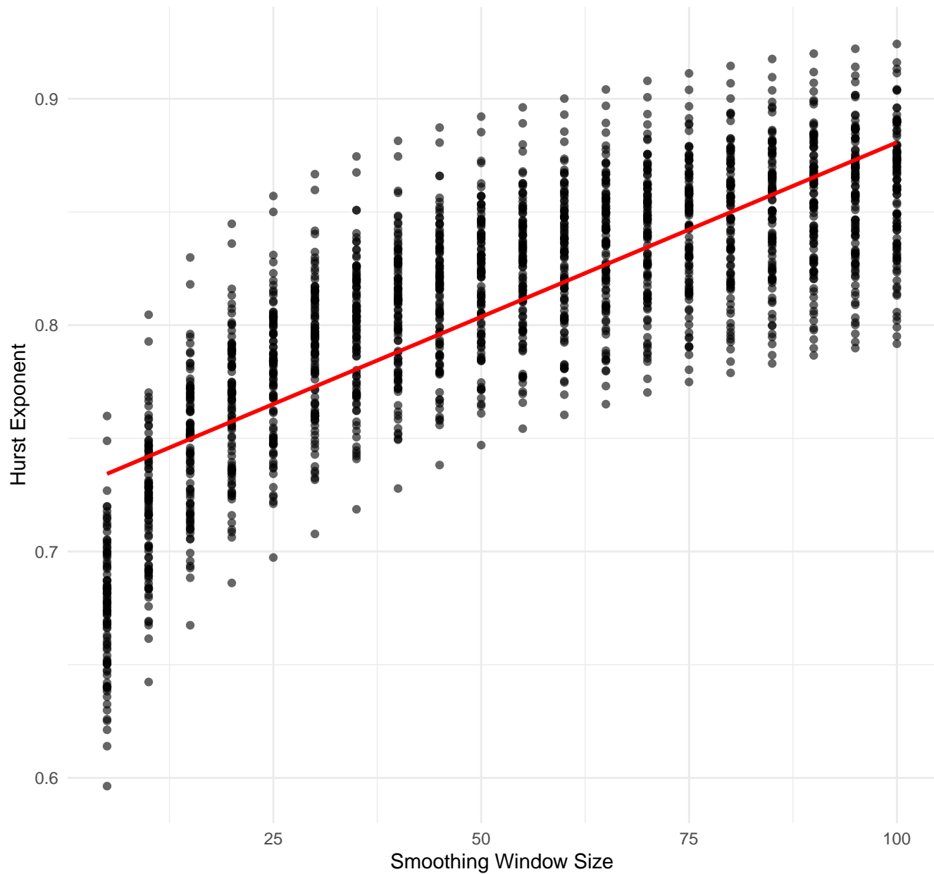
Hurst Exponent vs. Smoothing Window Size Correlation = 0.92
