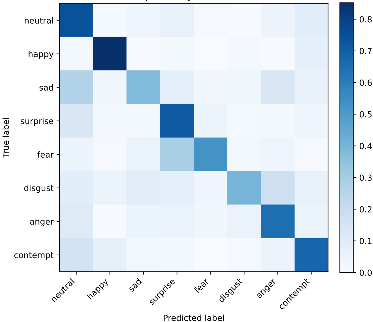
Confusion Matrix (Layer3+Layer4+FC Fine-tuned ResNet-50)
