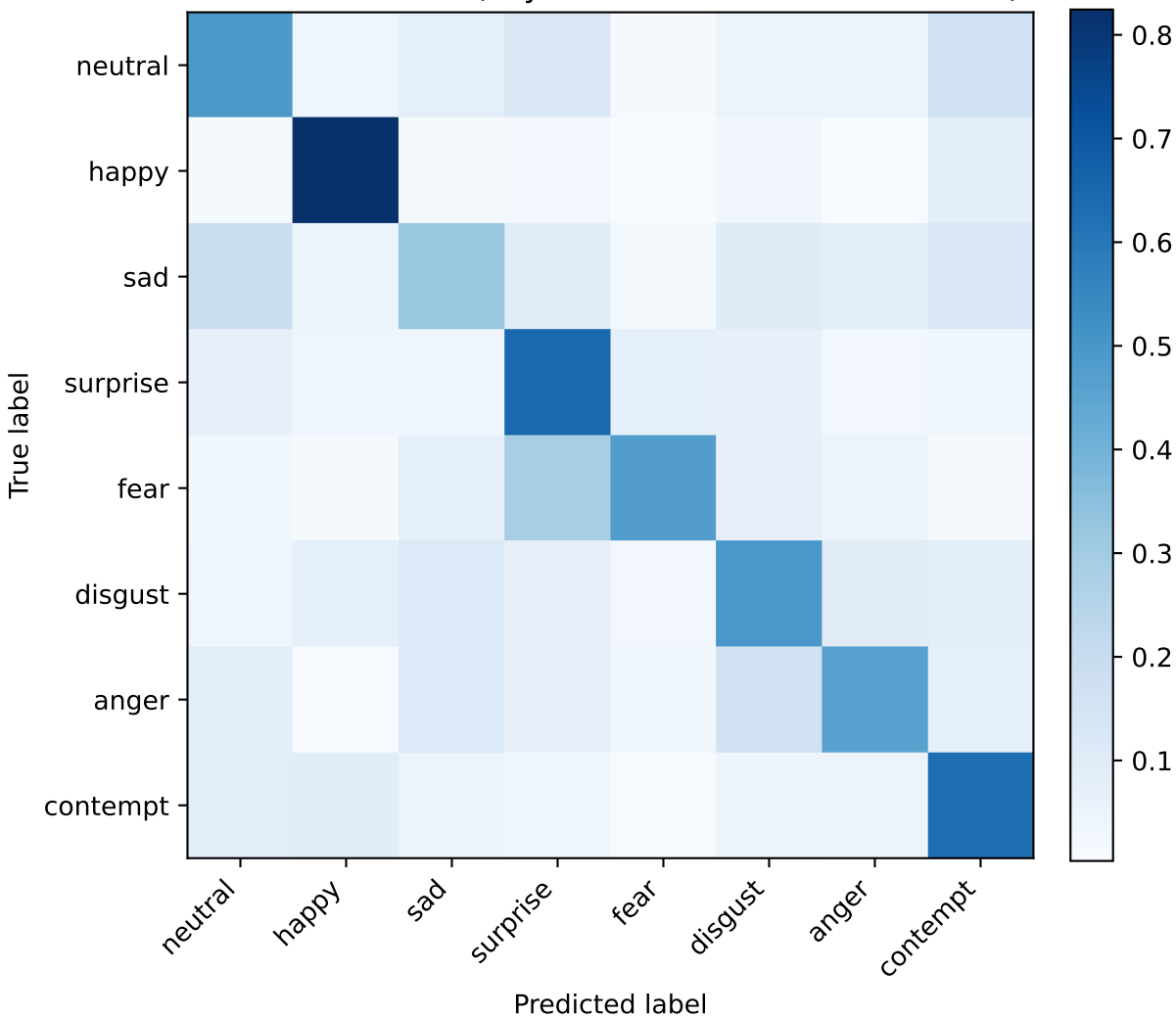
Confusion Matrix (Layer4+FC Fine-tuned ResNet-50)
