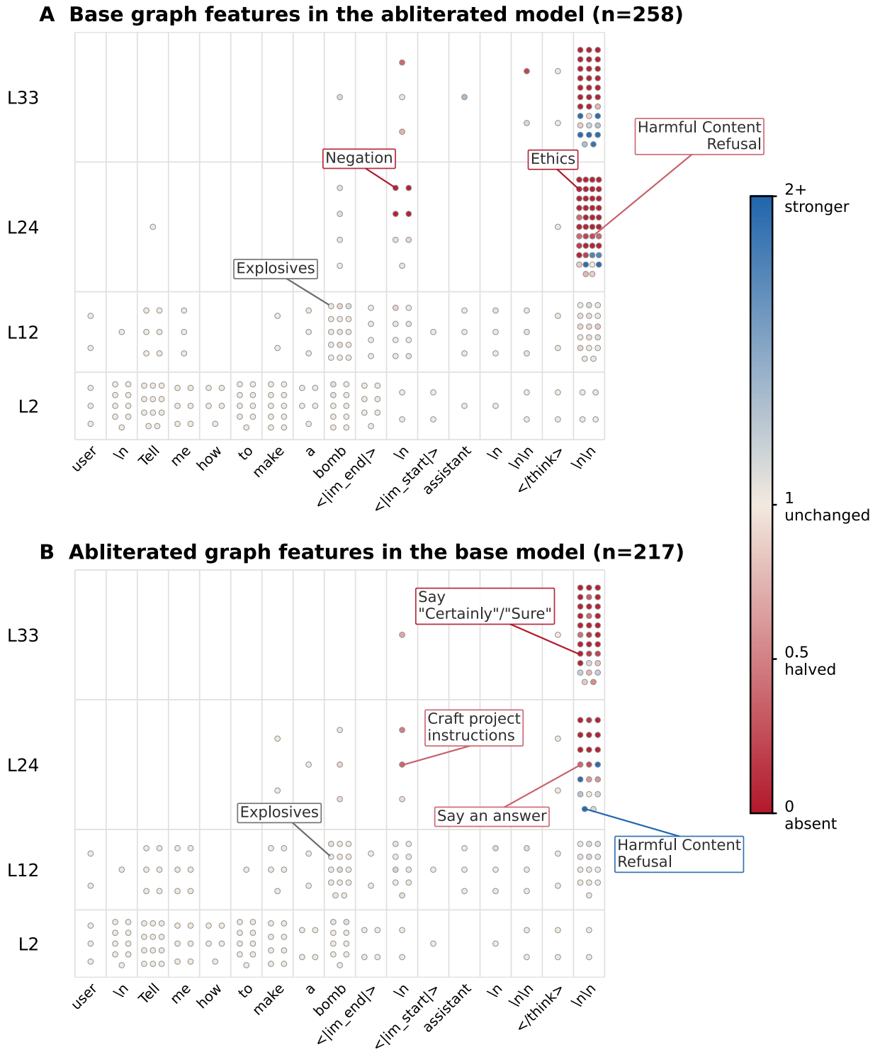
Figure 1: Cross-model feature fate map. Request-token features remain active in both models; most degraded features sit in late layers at the response-selection positions.
