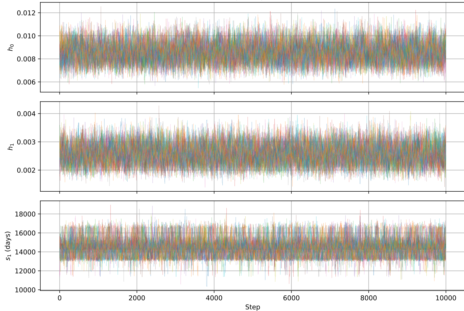
emcee trace plots (production run)
