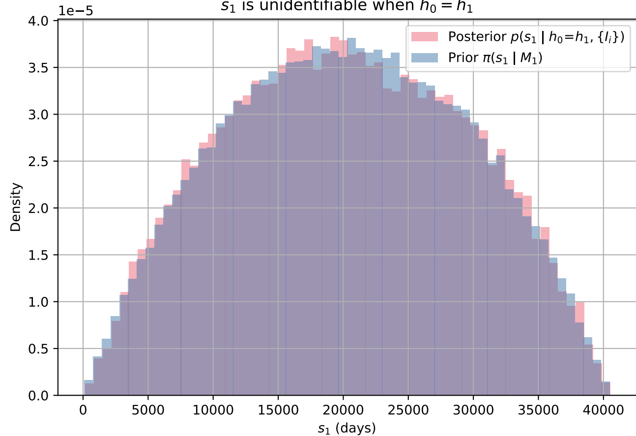
s_1 is unidentifiable when h_0 = h_1
