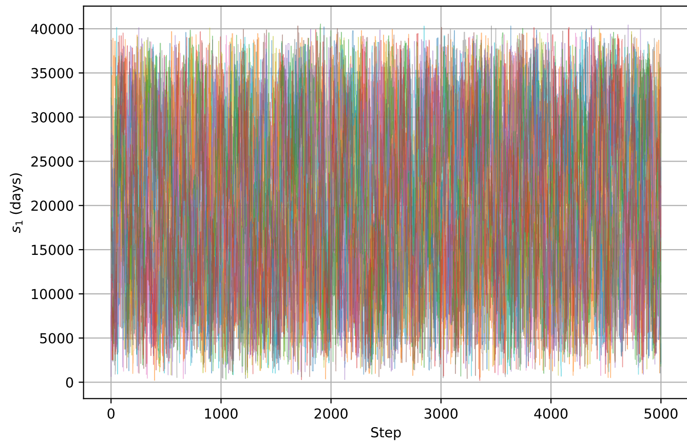
Trace of s_1 under h_0 = h_1 constraint
