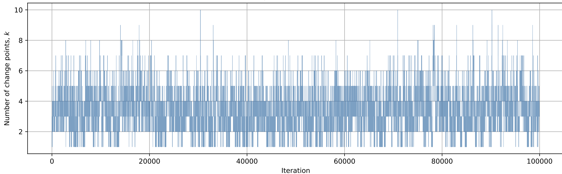
Posterior distribution on model index k
