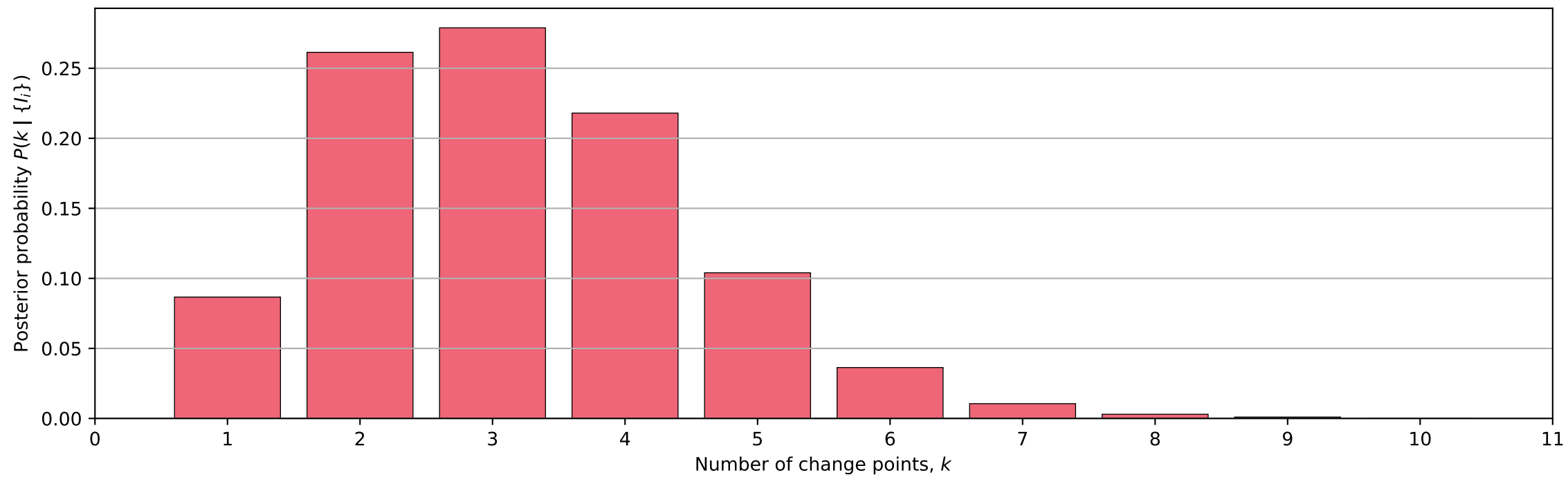
Posterior distribution on model index k
