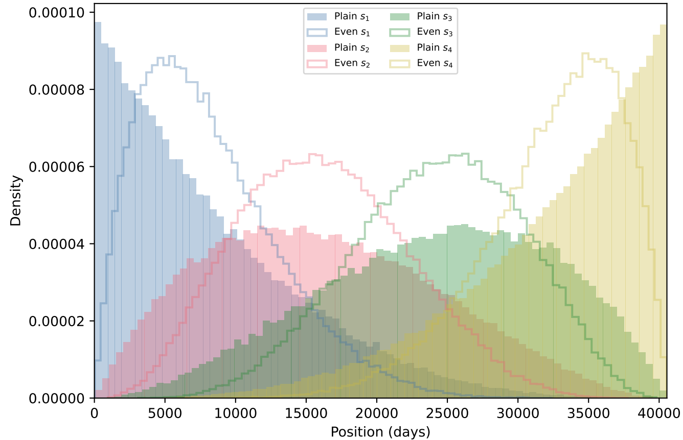
Marginal change-point densities ( k = 4 )
