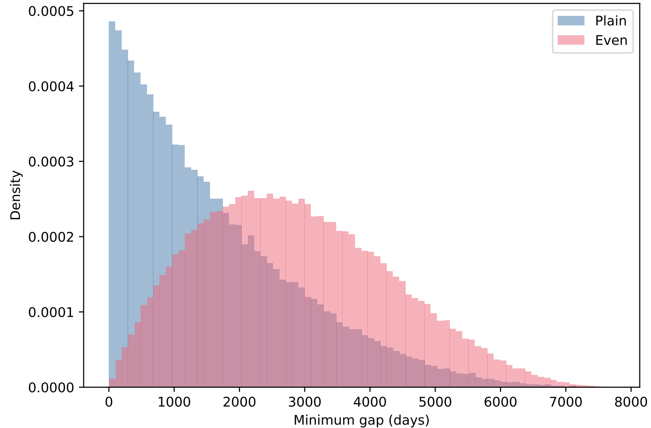
Distribution of minimum gap ( k = 4 )
