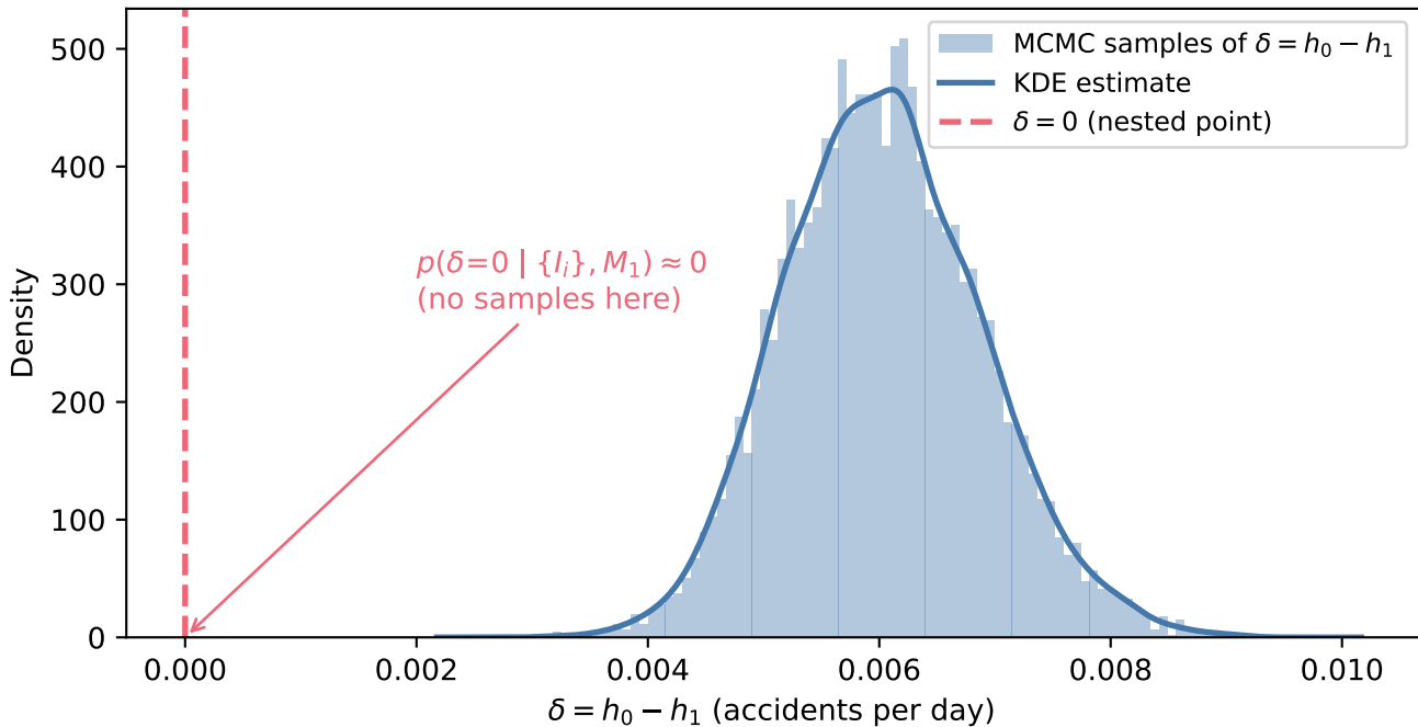
Savage-Dickey difficulty: posterior on \delta under M_1
