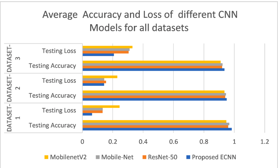
Fig. 11. Comparison of Average Accuracy and Loss of Proposed ECNN model with state of the art CNN models.
