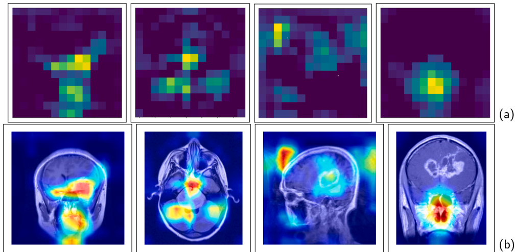
Fig. 7. Performance of The suggested fine-tuned EfficientNetV2S (a)attention map of brain tumor image sample (b)Grad-CAM visualization of MRI image samples.
