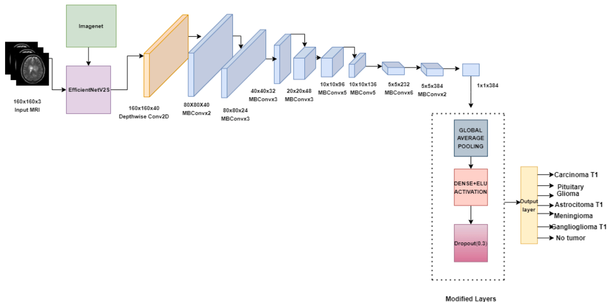
Fig. 3. Block diagram of the proposed fine-tuned ECNN model.
