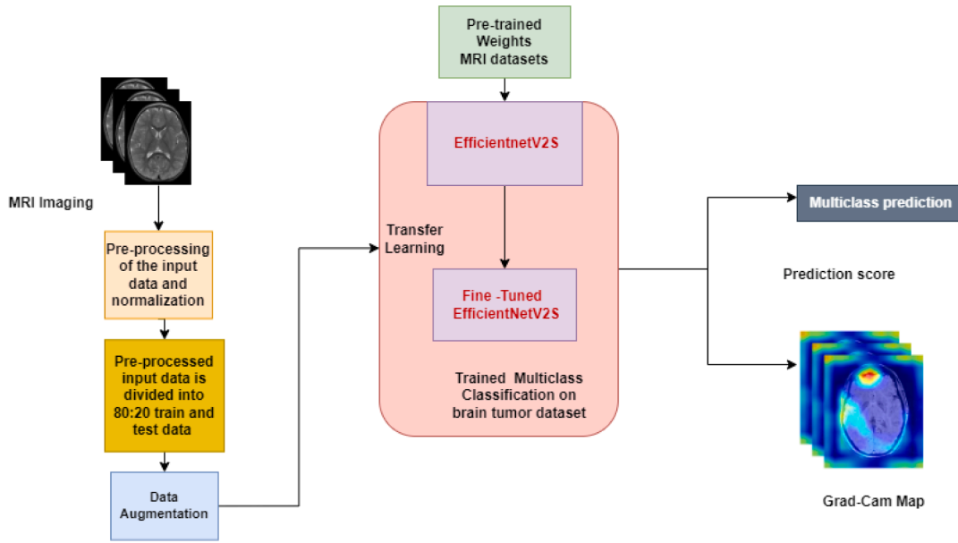
Fig. 1. The proposed framework for brain tumor detection using Grad-CAM visualization mechanism and transfer learning technique.
